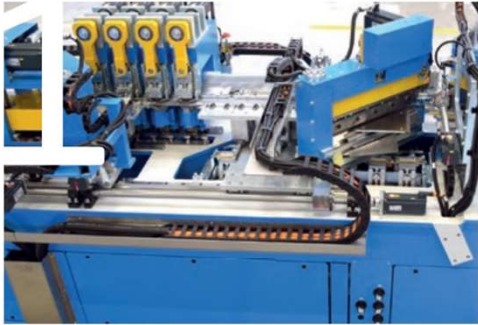
Core manufacturing — Core cutting lines
