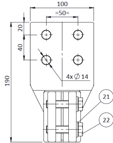
CONNECTION DETAILS
